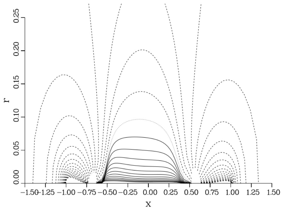
Figure 1: Plot of Contours Around Transonic Shock Free Body
