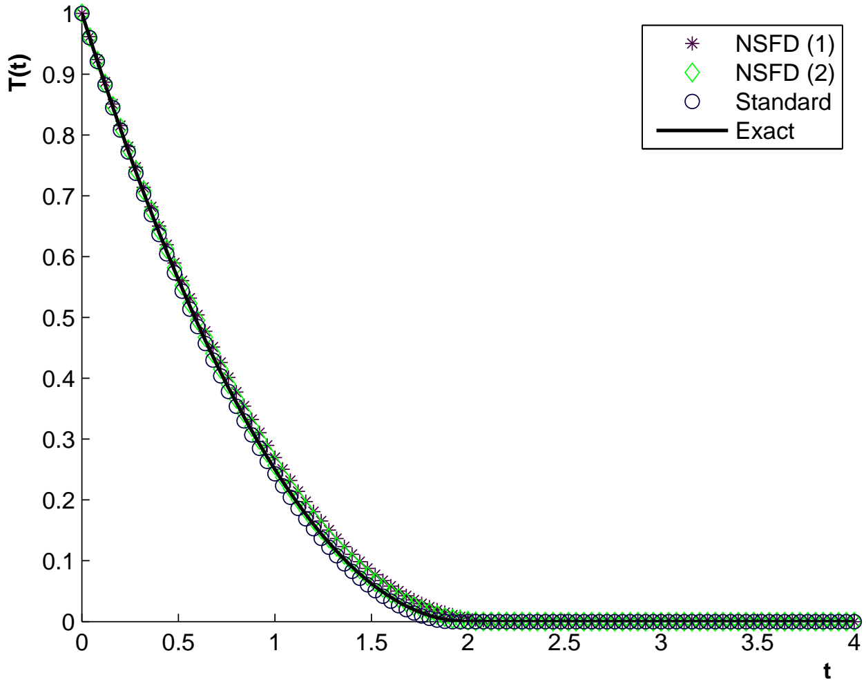
Figure 2: Comparison of NSFD(1), NSFD(2), the standard scheme, and the exact scheme for Equation (4).
