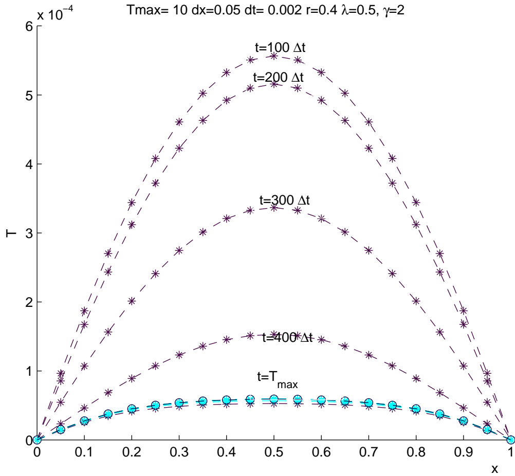
Figure 6: Plot of the differences between the standard scheme and the NSFD(1) scheme.
