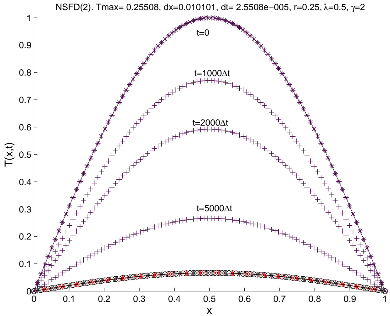
Figure 4: Plots of the NSFD(2) scheme at various times.
