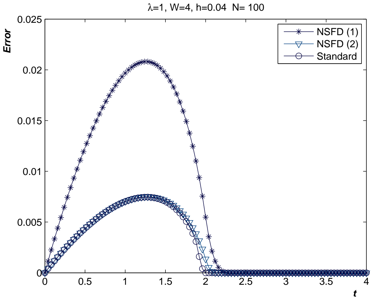
Figure 3: Plot of the differences between the NSFD(1), NSFD(2), the standard scheme, and the exact FD scheme
