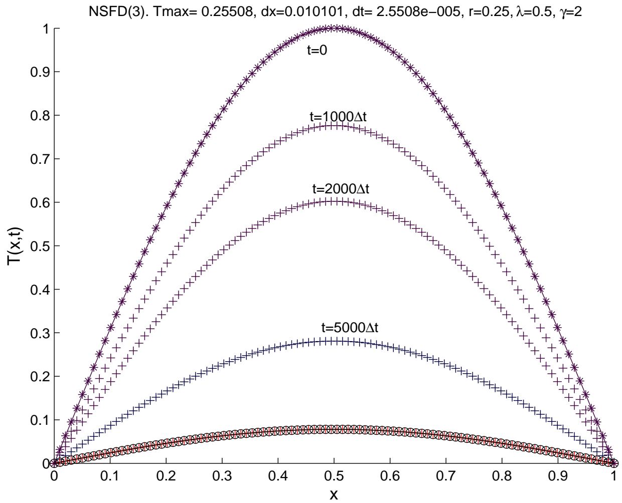
Figure 5: Plots of the NSFD(3) scheme at various times
