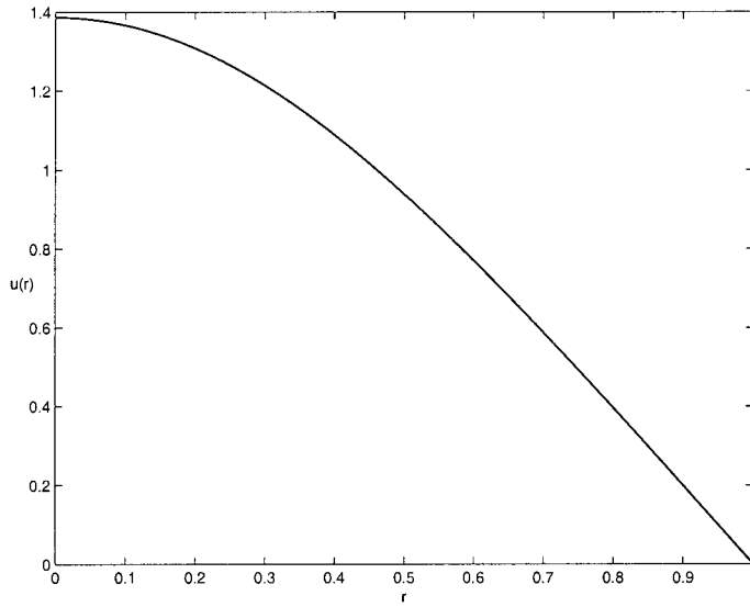
FIG. 3. Exact solution of the Bratu-Gelfand problem when \lambda = 2 .
