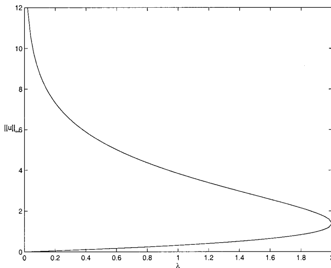
FIG. 2. Maximum value of u(r) versus \lambda depicting the turning point at \lambda = 2 .
