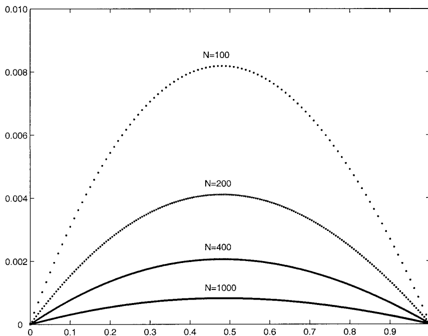
FIG. 4. Numerical error versus r for standard method when \lambda = 1 .
