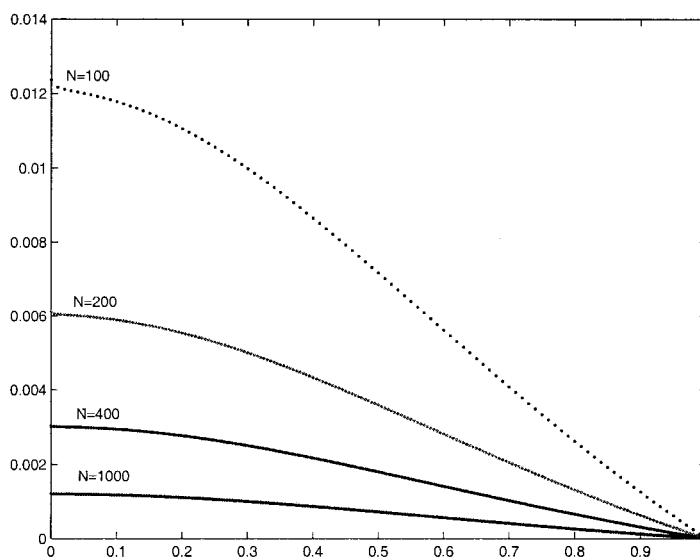
FIG. 6. Numerical error using Mickens finite differences with N = 100, 200, 400, and 1000 for \lambda = 2 .
