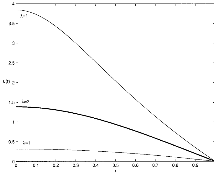
FIG. 1. Exact solutions to the Bratu-Gelfand problem when \lambda = 1 (bifurcated) and \lambda = 2 (unique).
