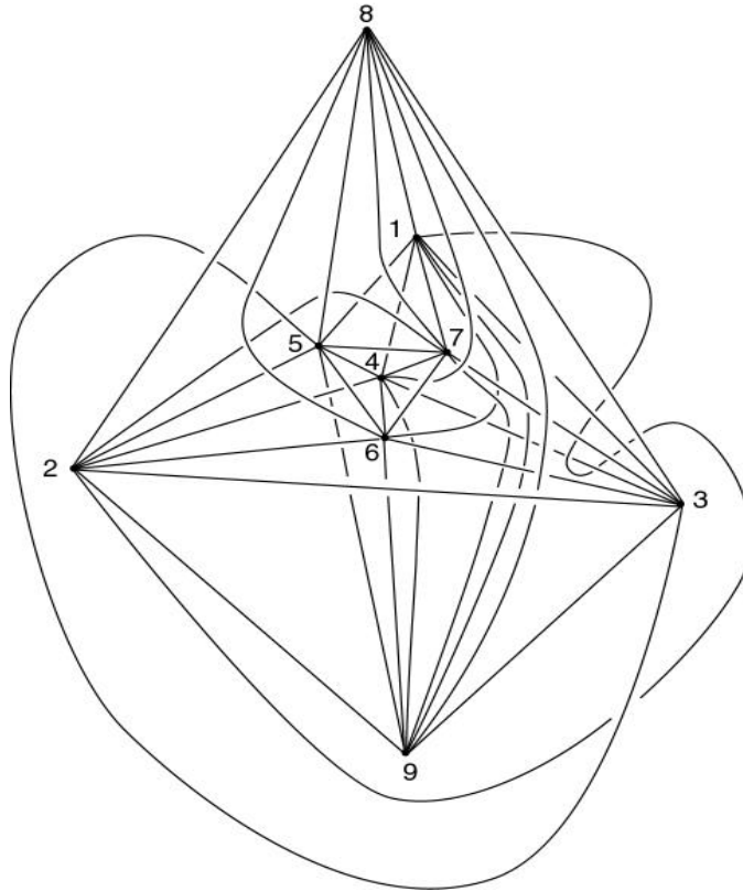
FIGURE 1. This embedding of K_9 has no triple link
