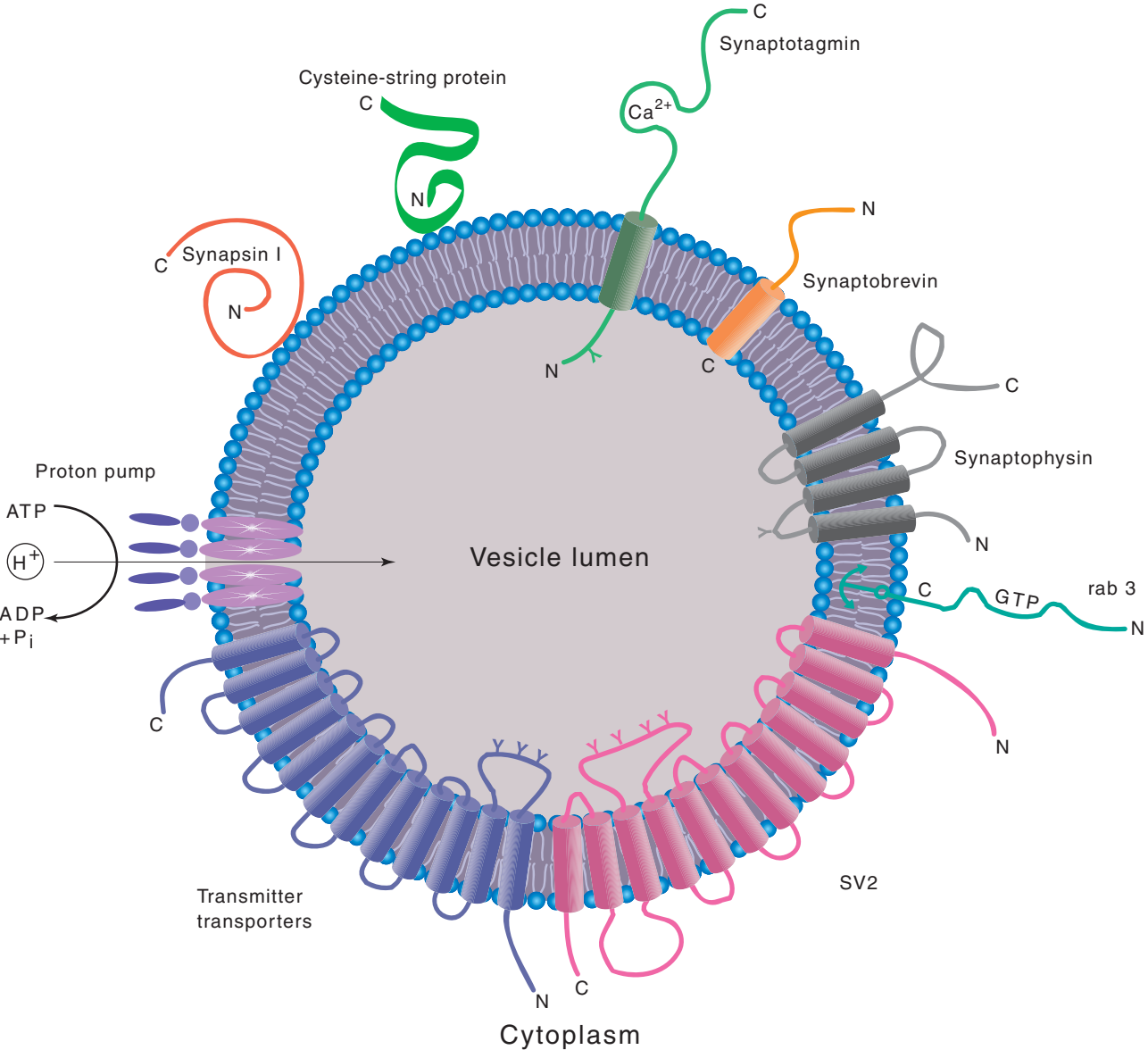
FIGURE 8.4 Schematic representation of the structure and topology of the major synaptic vesicle membrane proteins (see also Table 8.1). N, amino terminal; C, carboxy terminal.
