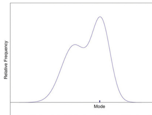
Figure 2.2.3: Mode
