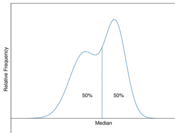
Figure 2.2.1: The Median
