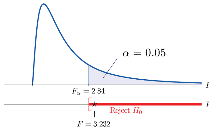
Figure 11.4.1: Rejection Region
