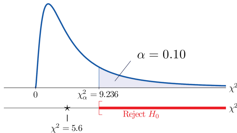
Figure 11.2.1: Balanced Die
