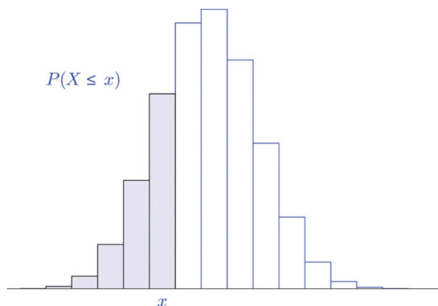
Figure 4.3.3: Cumulative Probabilities
