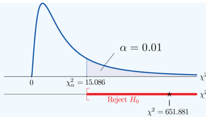
Figure 11.2.2: "Example 11.2.1"
