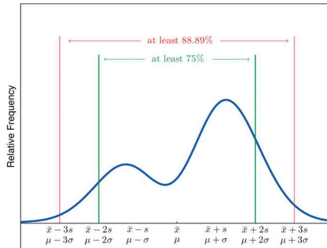
Figure 2.5.4: Chebyshev's Theorem
