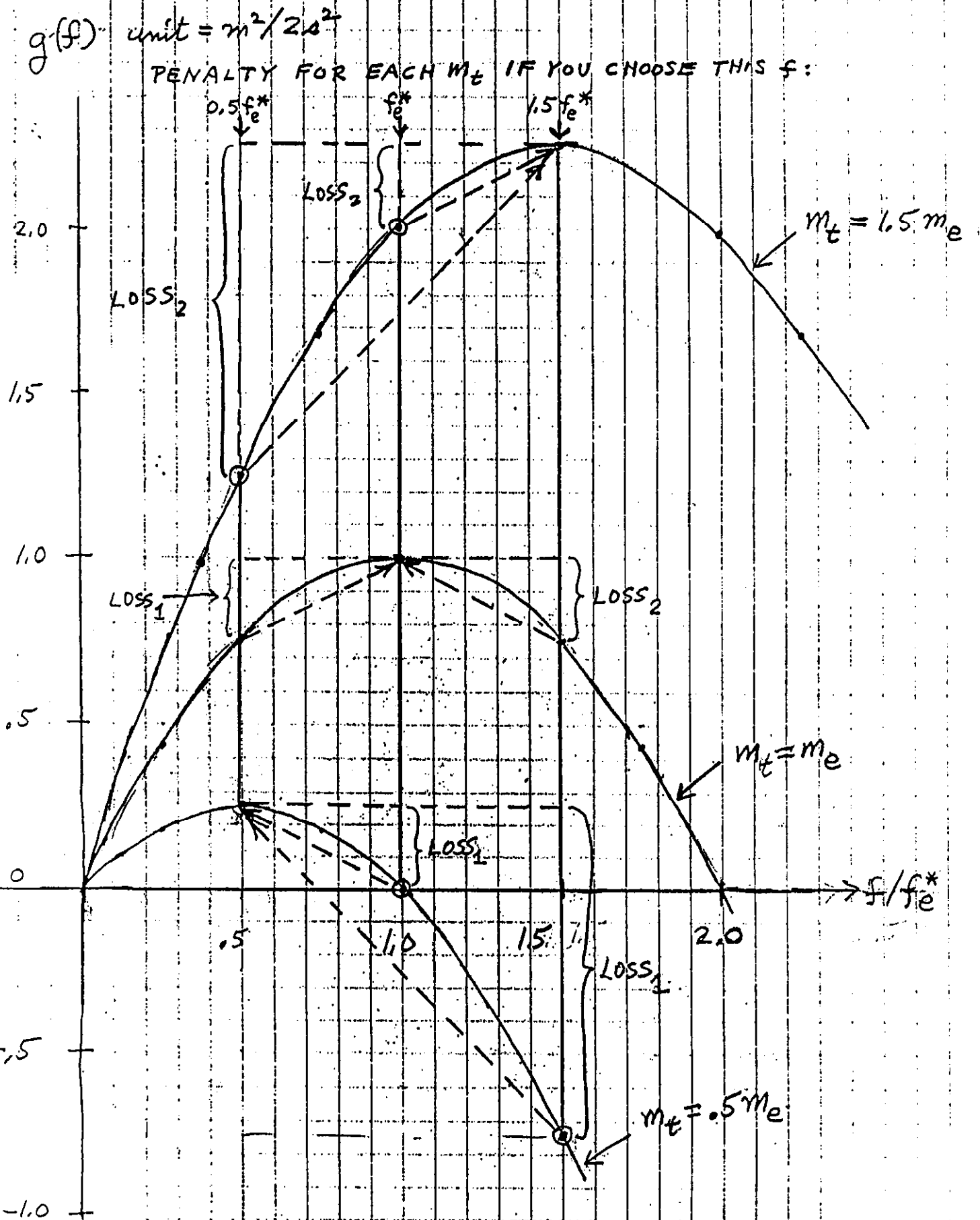
FIGURE 5. Penalties for choosing f = f_e \neq f^* = f_t
