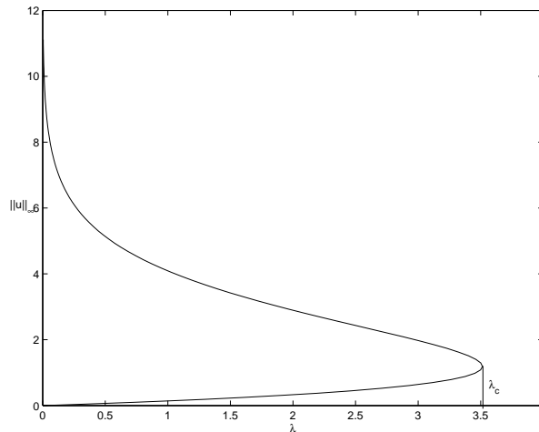
Figure 2: Bifurcated nature of the exact solution to the Bratu problem
